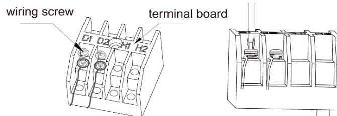
Fig 7 Communication terminal
