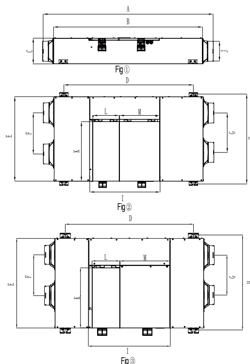
Fig ② is the access panel front view of FHBQGL-D3.5DA-T and FHBQGL-D5DA-T, Fig ③ is the access panel front view of FHBQGL-D1.5DA-T and FHBQGL-D2.5DA-T Fig 1 Size label
