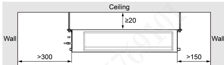
(7) Middle Static Pressure Duct Type Indoor Unit GMV-ND**PMS/A1-T Series
