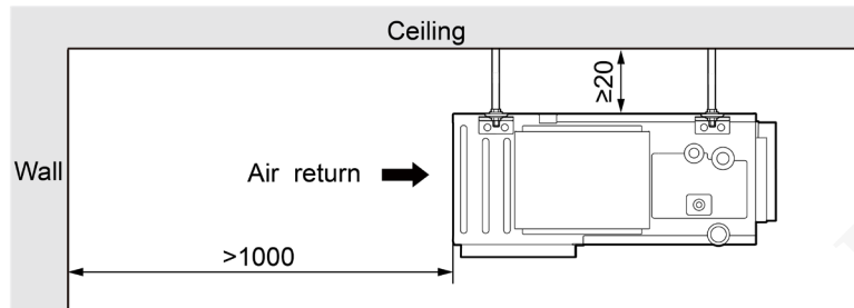
(7) Middle Static Pressure Duct Type Indoor Unit GMV-ND**PMS/A1-T Series
