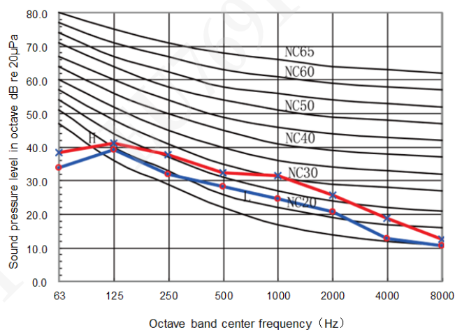
Model GMV-ND90~112PLS/C-T
