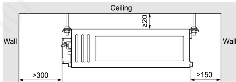
(6) High Static Pressure Duct Type Indoor Unit GMV-ND**PHS/D-T Series
