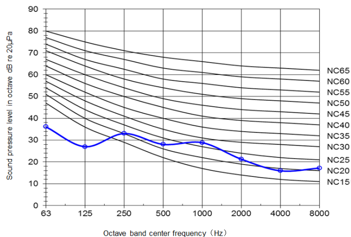
Model GMV-ND71PLS/B1-T
