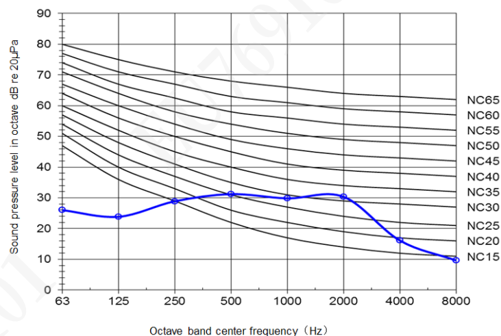
Model GMV-ND32~36PLS/B1-T
