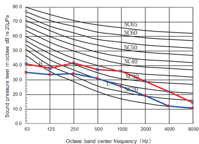
Model GMV-ND125~140PLS/C-T
